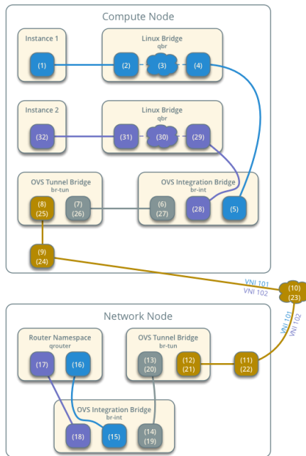
Open vSwitch - Self-service Networks Network Traffic Flow - East/West Scenario 2
