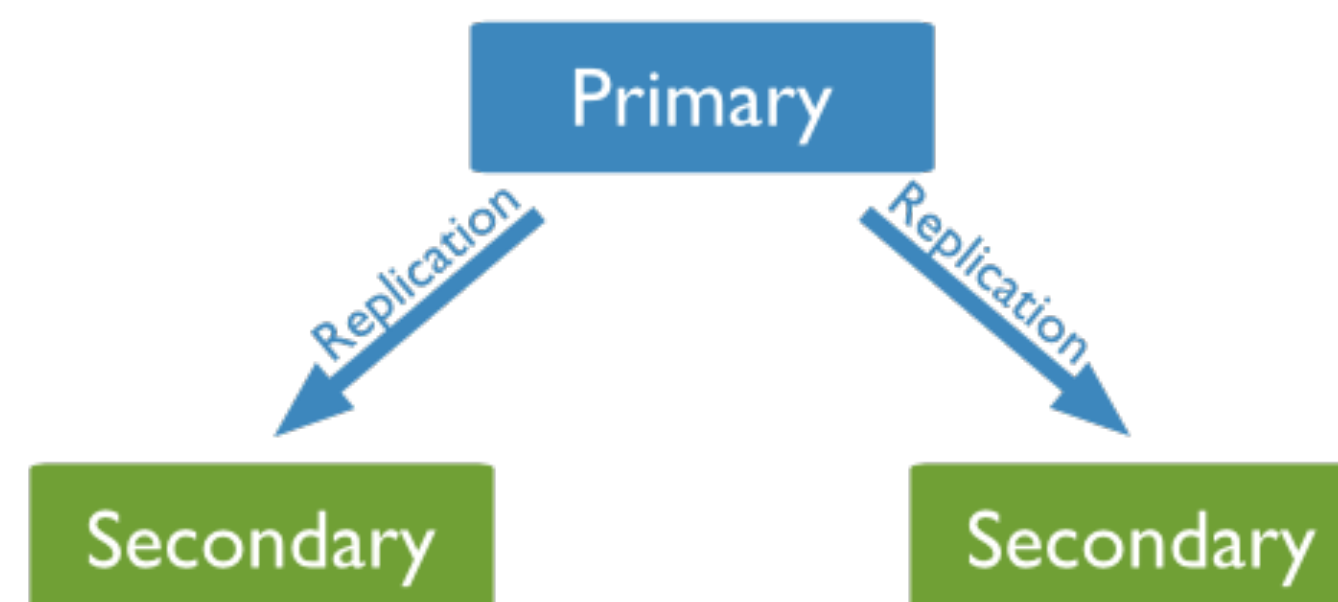
Replica set
