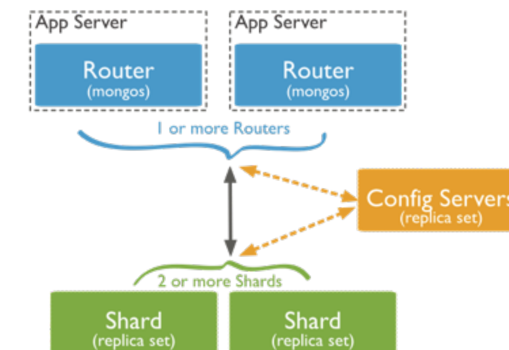
Sharded cluster
