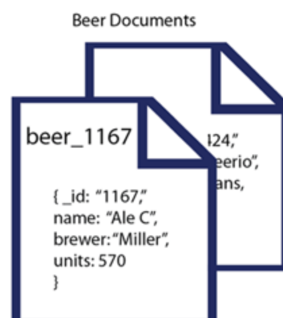
Document model
