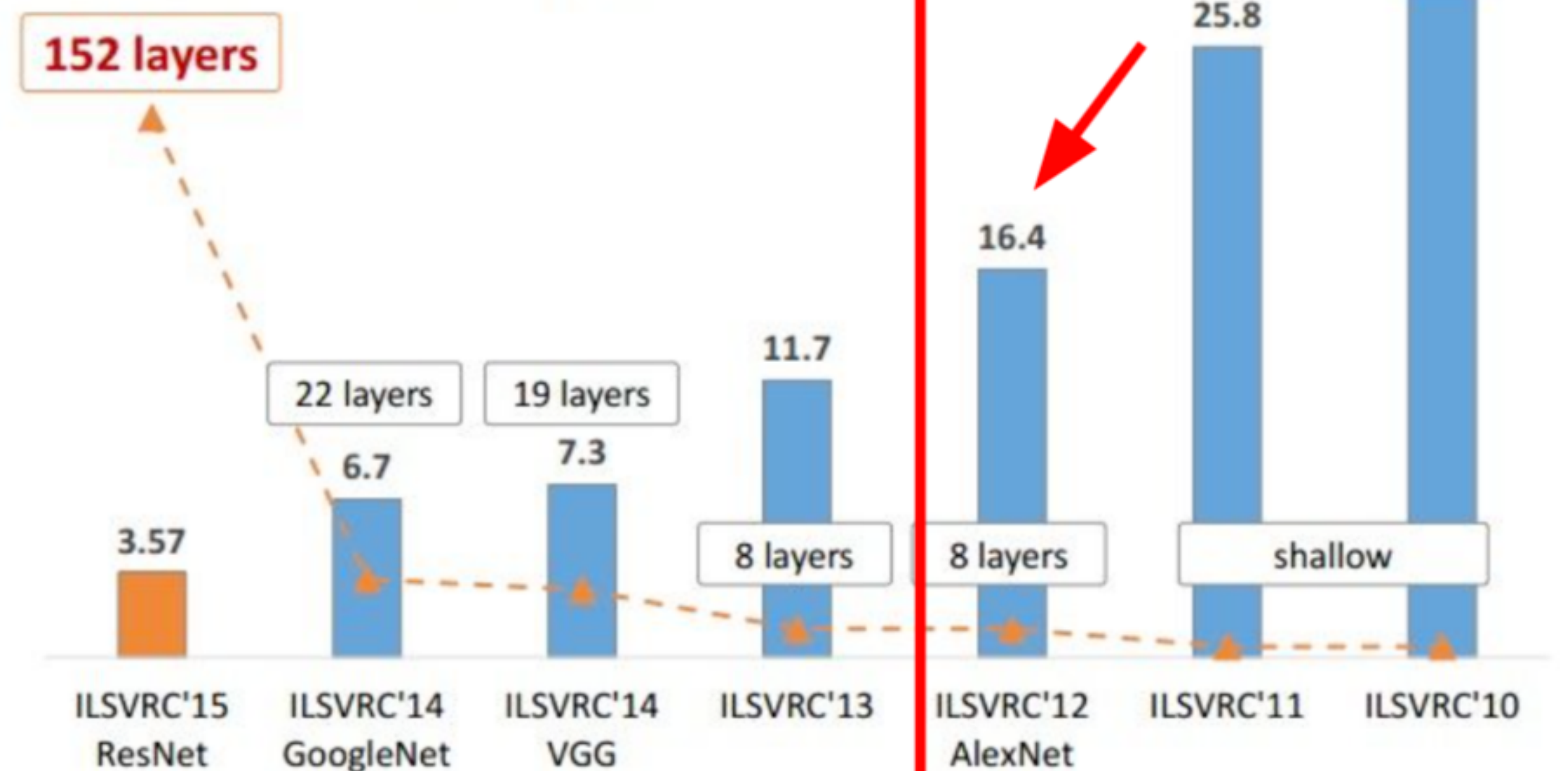
ImageNet Classification top-5 error (%)
